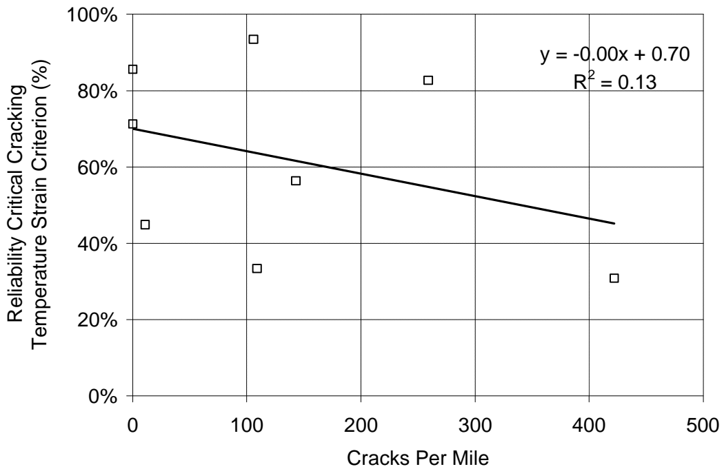
FIGURE 3.11 Correlation Between Reliability of Critical Cracking Temperature – Stress Criterion and Field Cracking
