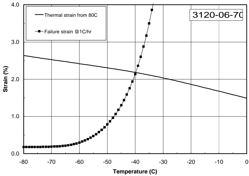
FIGURE 3.7 Cracking Temperature, Strain Criterion (3120-06-70)
