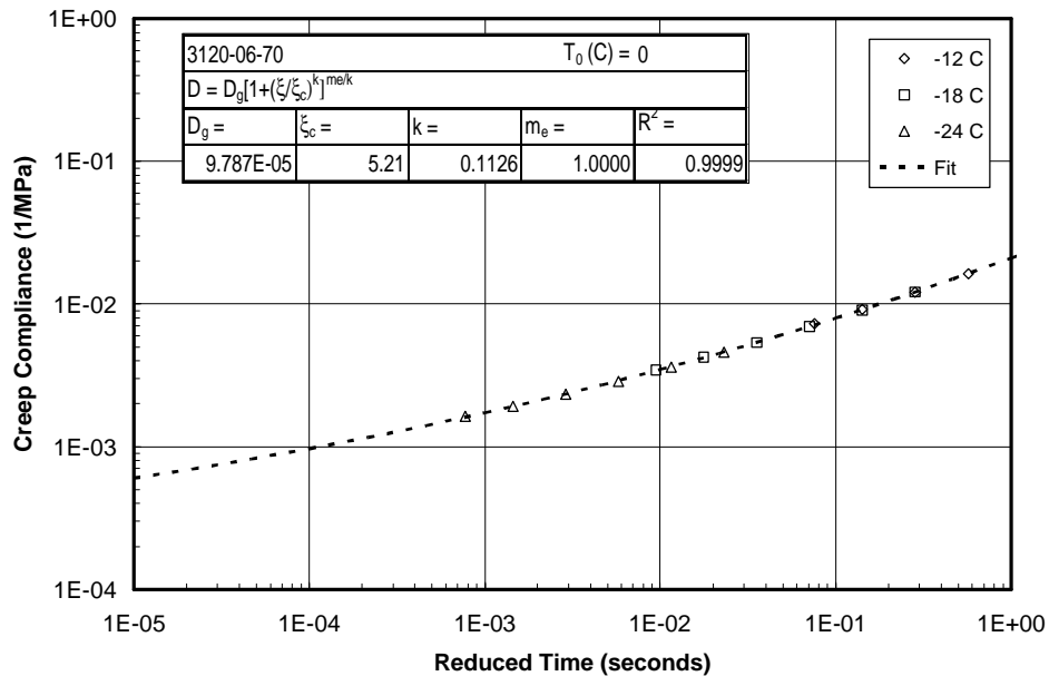
FIGURE 3.2 Creep Compliance Master Curve from BBR Data (3120-06-70)
