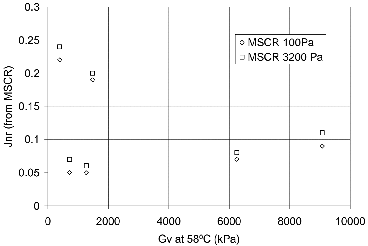
FIGURE 4.2 G_v (at 58°C) v/s J_{nr} , RTFO Residue
