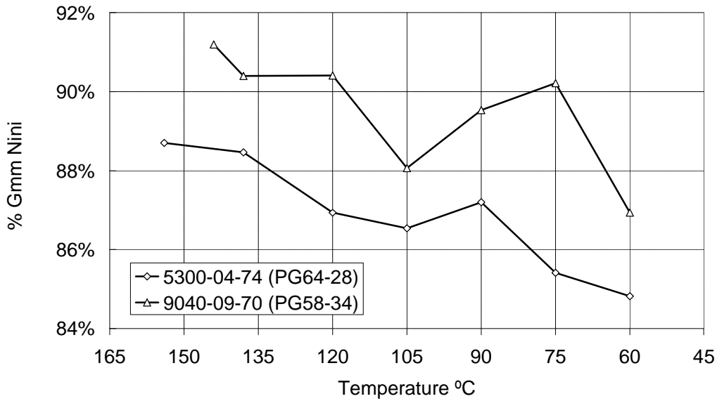
FIGURE 1.6 %Gmm at Nini versus Temperature Mixtures for Projects 5300-04-74 and 9040-09-70 (600 kPa)
