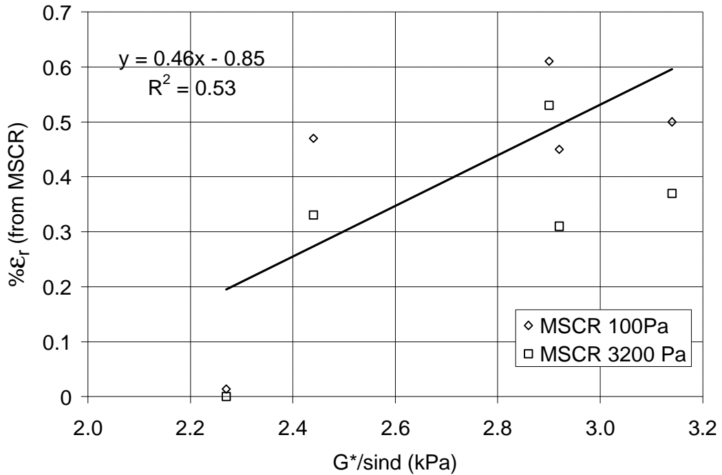
FIGURE 4.4 G^*/\sin\delta v/s % \epsilon_r , RTFO Residue
