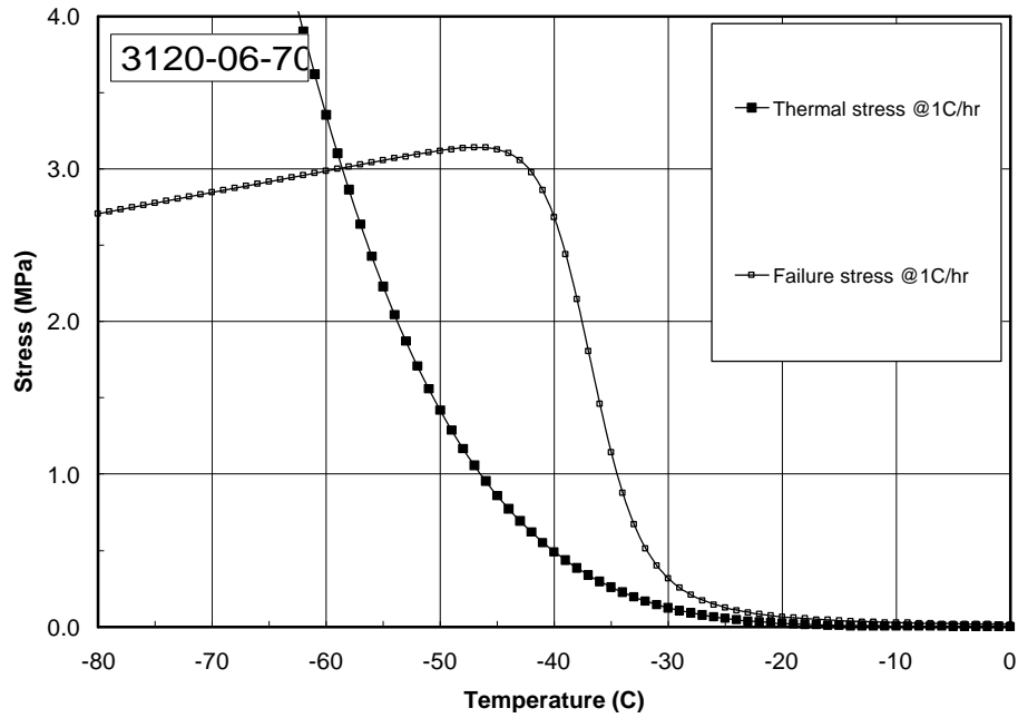
FIGURE 3.6 Cracking Temperature, Stress Criterion (3120-06-70)
