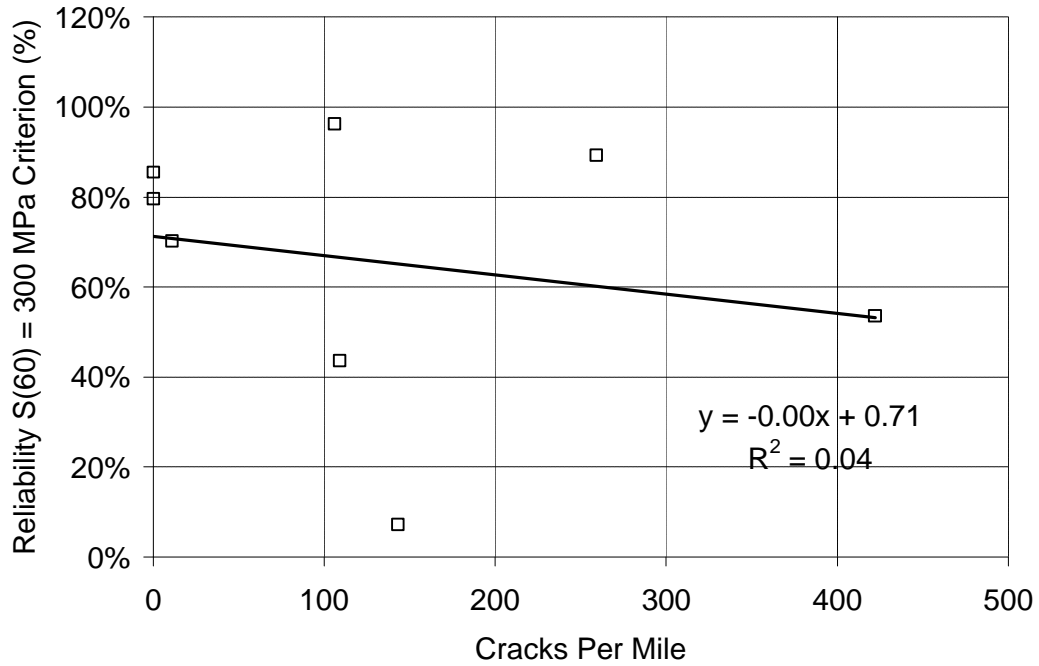
FIGURE 3.10 Correlation Between Reliability of Temperature for S(60) = 300 MPa Criterion and Field Cracking
