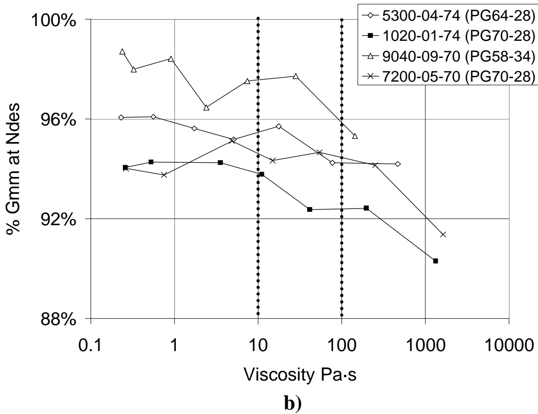
FIGURE 1.8 %Gmm at Ndes versus Binder Viscosity (Lab Data)
