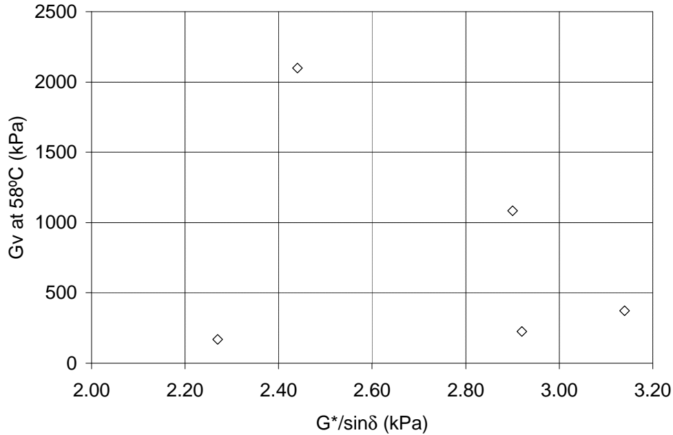
FIGURE 4.1 G^*/\sin\delta v/s G_v (at 58°C), RTFO Residue
