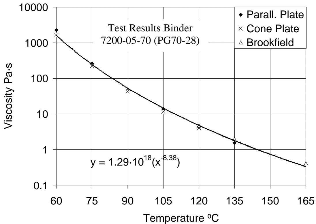
FIGURE 1.4 Viscosity Versus Temperature for binder 7200-05-70 (PG70-28)
