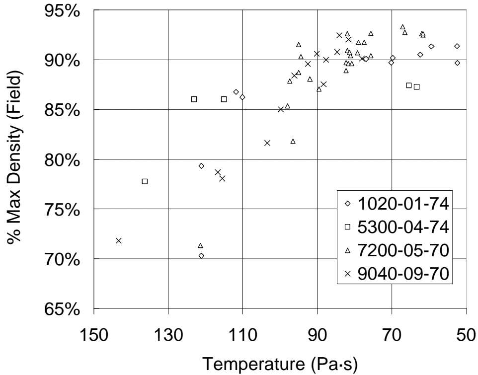
FIGURE 1.2 Field Density v/s Temperature, All Projects
