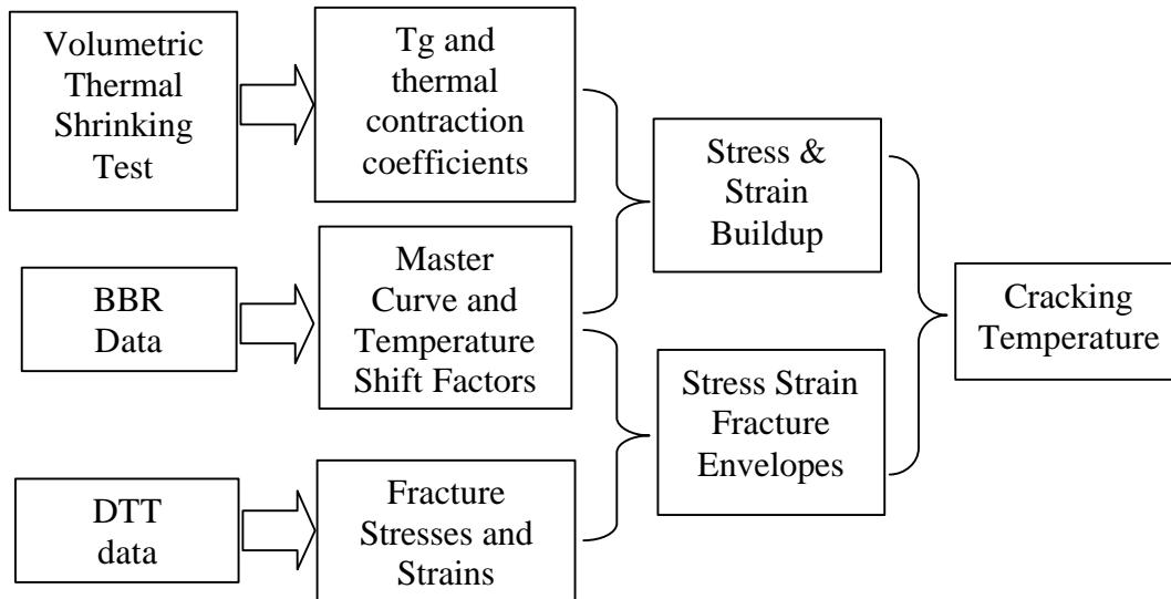
FIGURE 3.1 Flowchart for Determining Cracking Temperature
