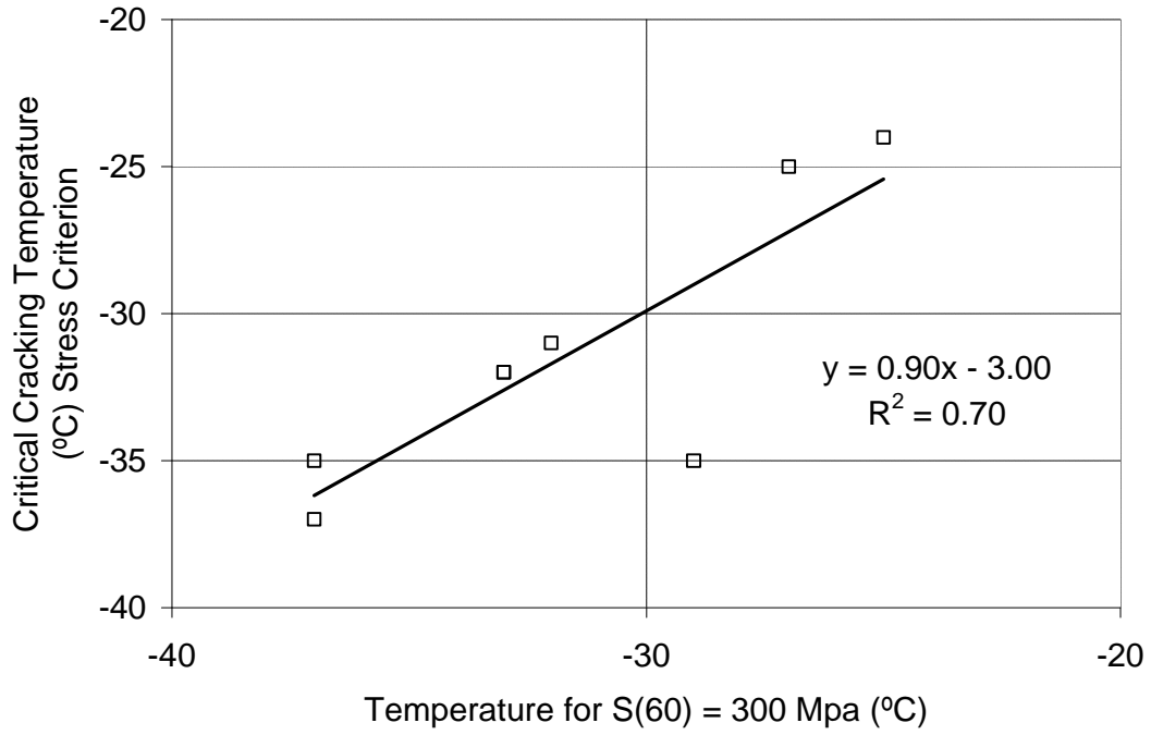
FIGURE 3.8 Correlation Between Critical Cracking Temperature - Stress Criterion and Temperature for S(60) = 300 MPa
