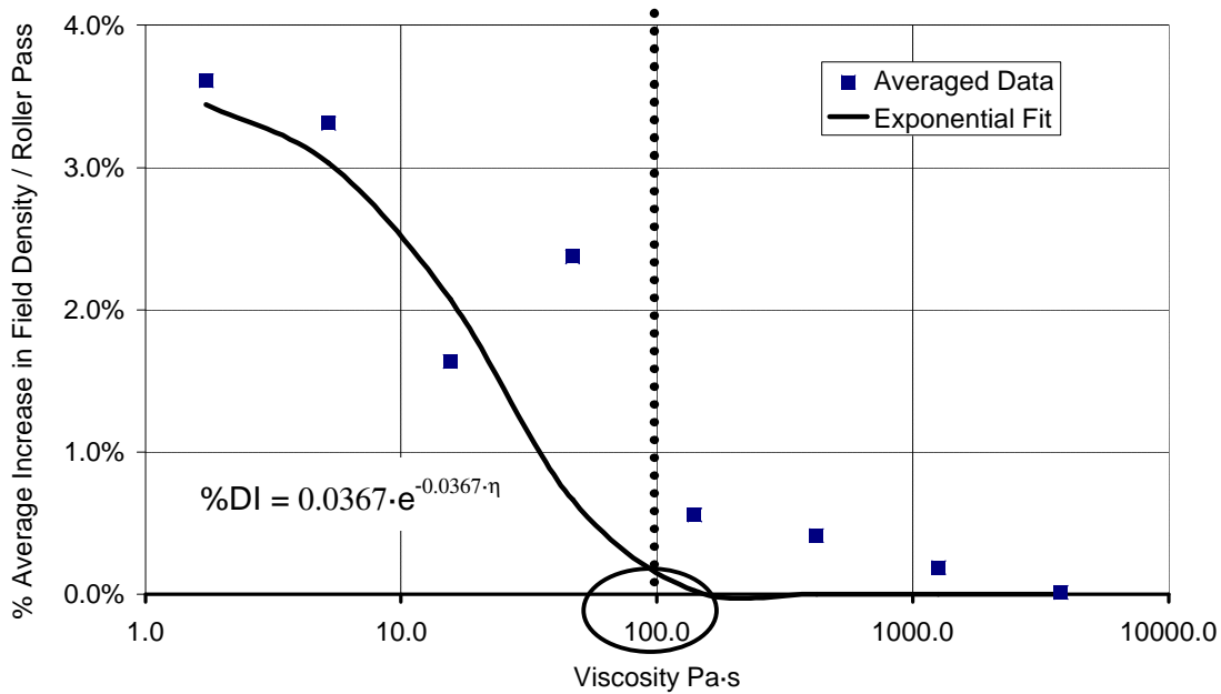
FIGURE 1.7 % Density Increase (%DI) versus Binder Viscosity (Field Data)
