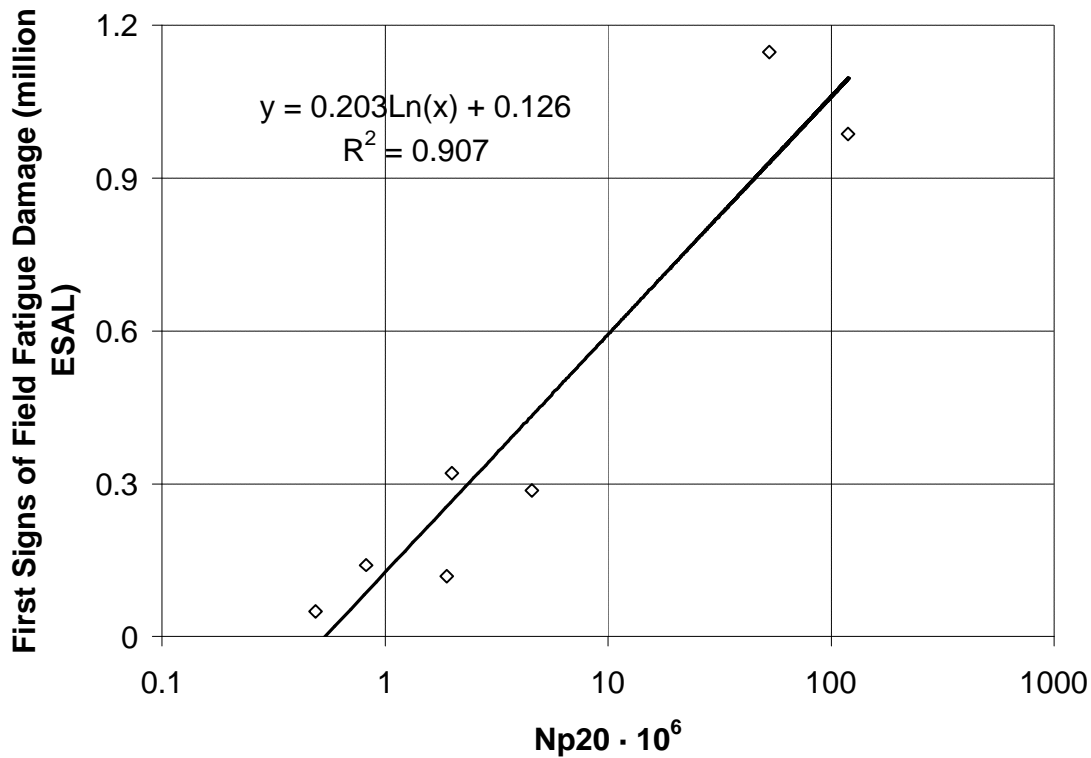
FIGURE 2.1 Binder N_{P20} Values v/s First Signs of Field Fatigue Damage
