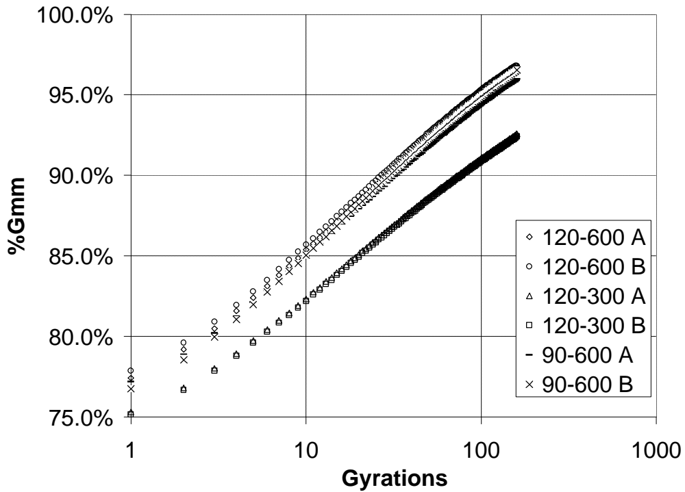
FIGURE 1.5 Compaction Curves Project 7200-05-70, 120°C and 90°C
