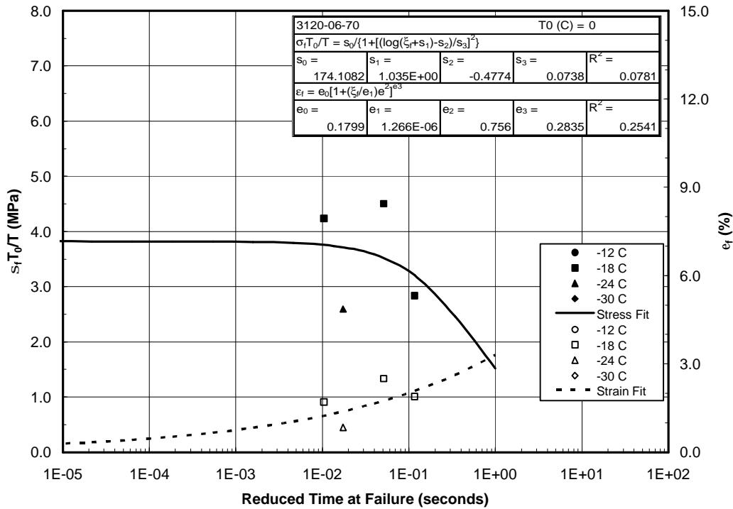
FIGURE 3.5 Fracture Curves (3120-06-70)
