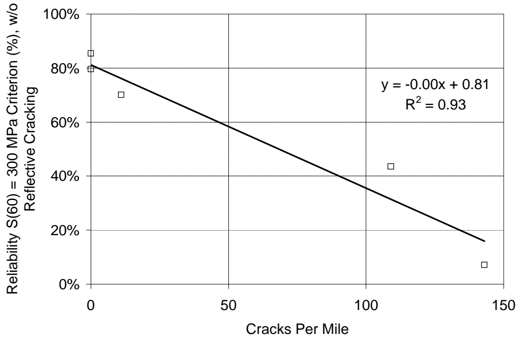
FIGURE 3.12 Correlation Between Reliability of Temperature for S(60) = 300 MPa Criterion and Field Cracking, Excluding Reflective Cracking
