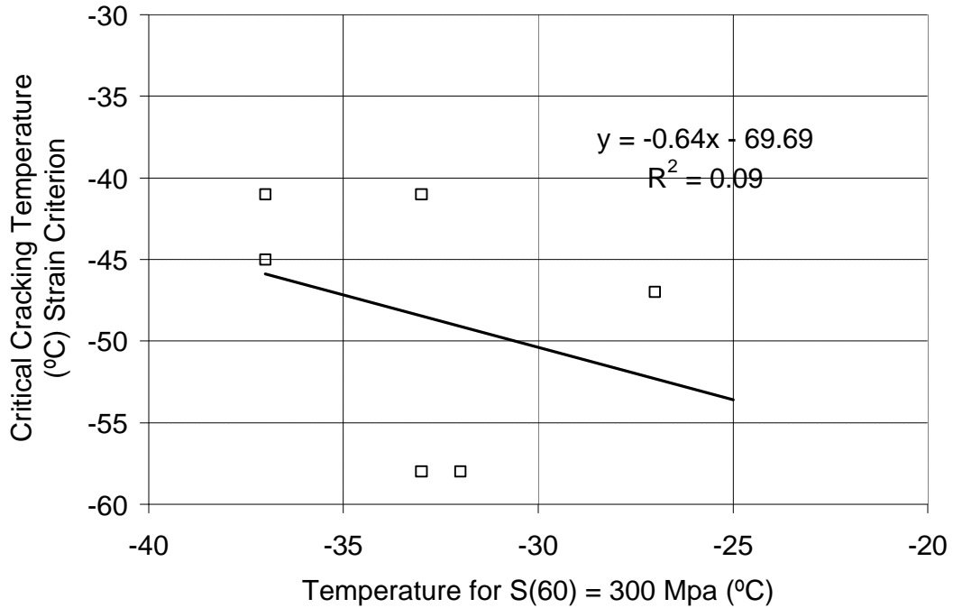
FIGURE 3.9 Correlation Between Critical Cracking Temperature - Strain Criterion and Temperature for S(60) = 300 MPa
