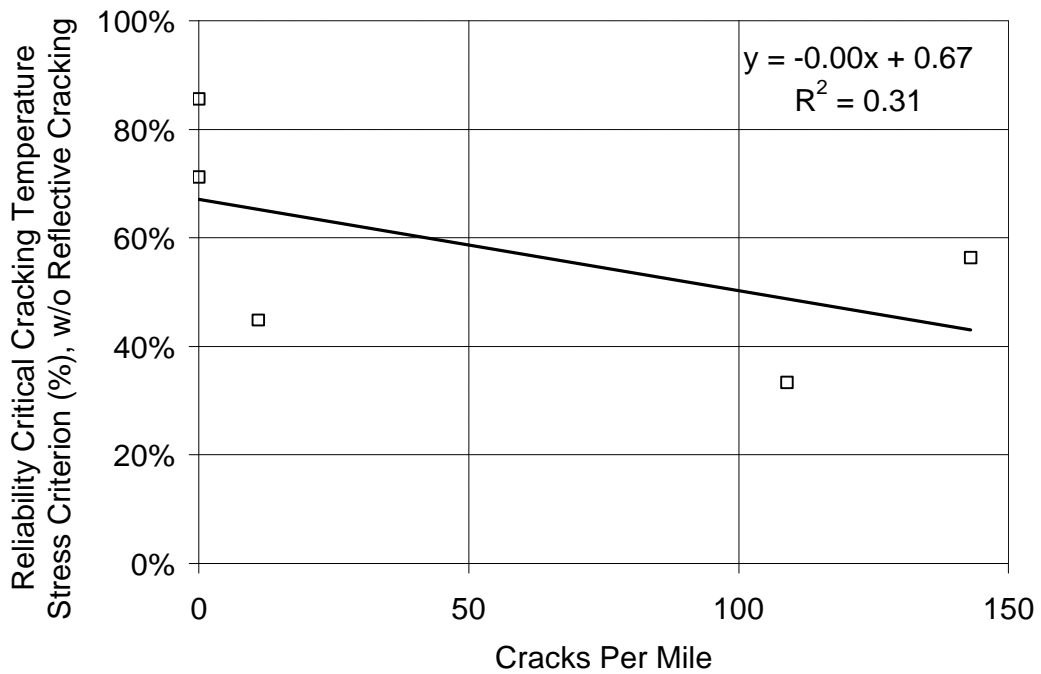
FIGURE 3.13 Correlation Between Reliability of Critical Cracking Temperature – Stress Criterion and Field Cracking, Excluding Reflective Cracking
