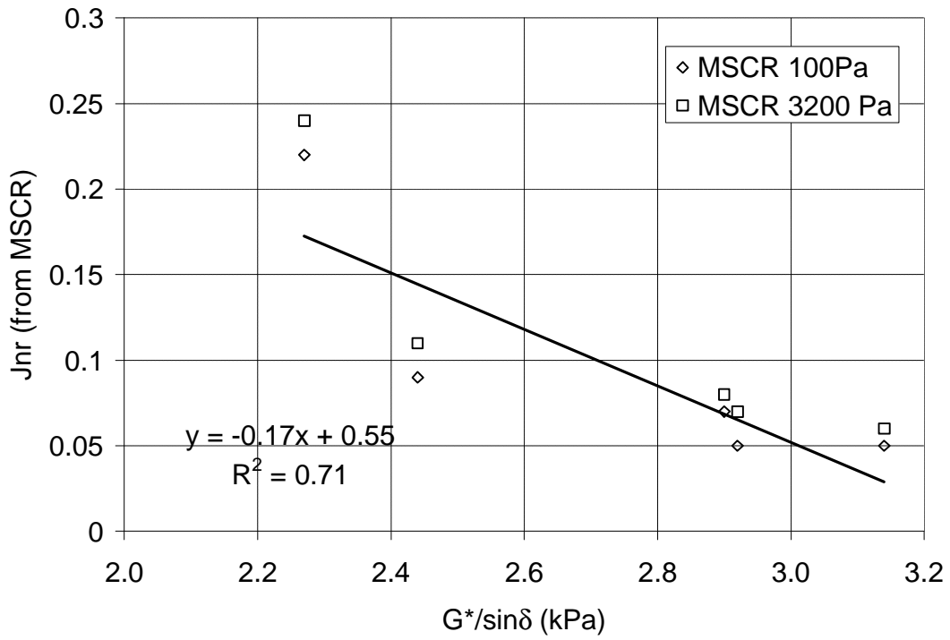
FIGURE 4.3 G^*/\sin\delta v/s Jnr, RTFO Residue
