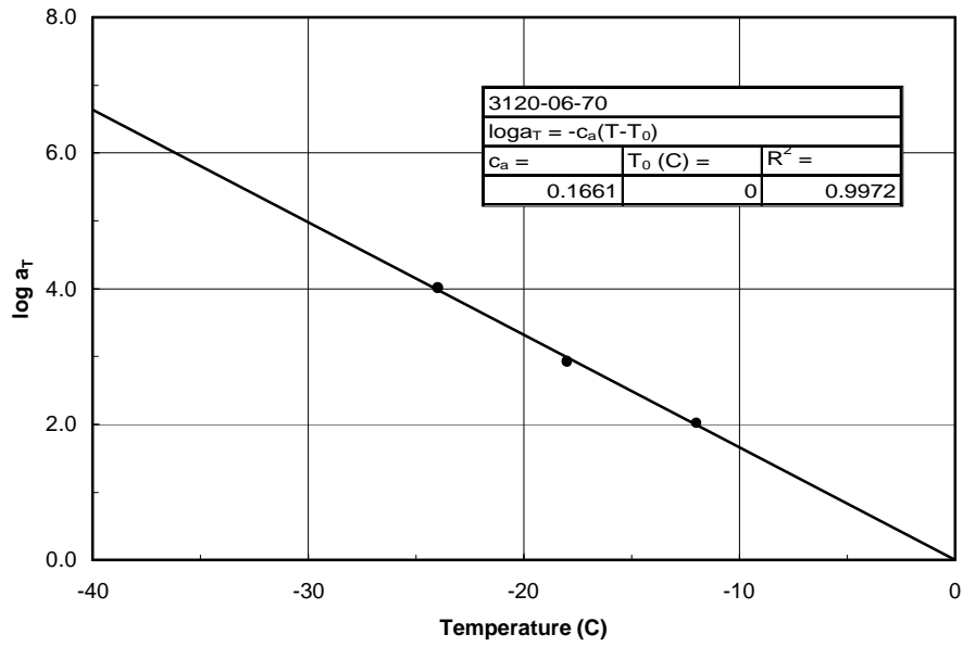
FIGURE 3.3 Temperature Shift Factor (3120-06-70)
