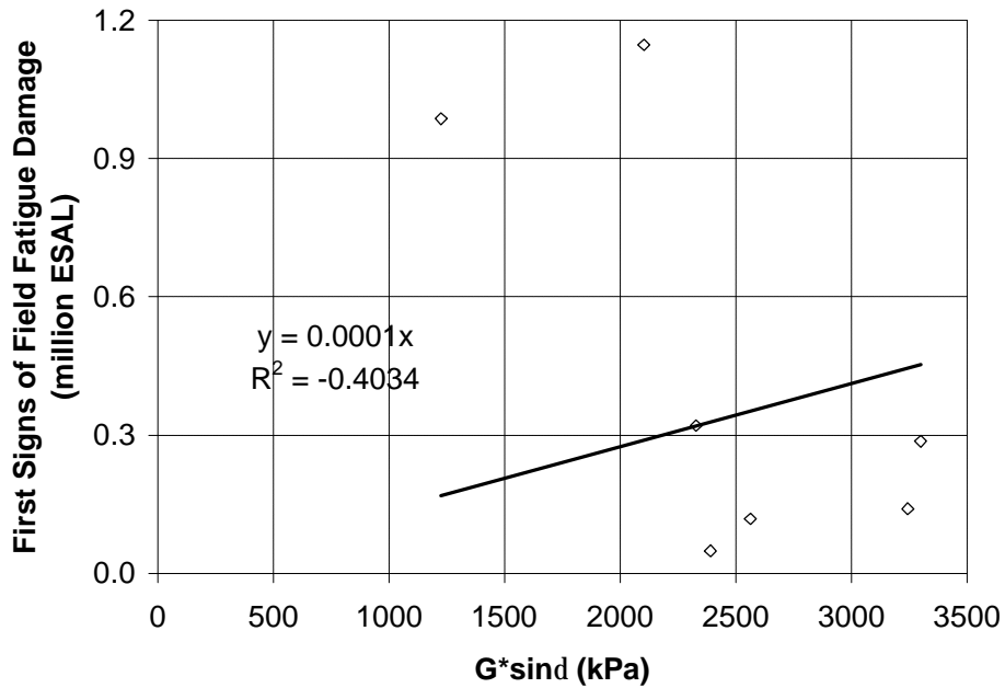
FIGURE 2.5 G \cdot \sin \delta v/s Field First Signs of Fatigue Damage
