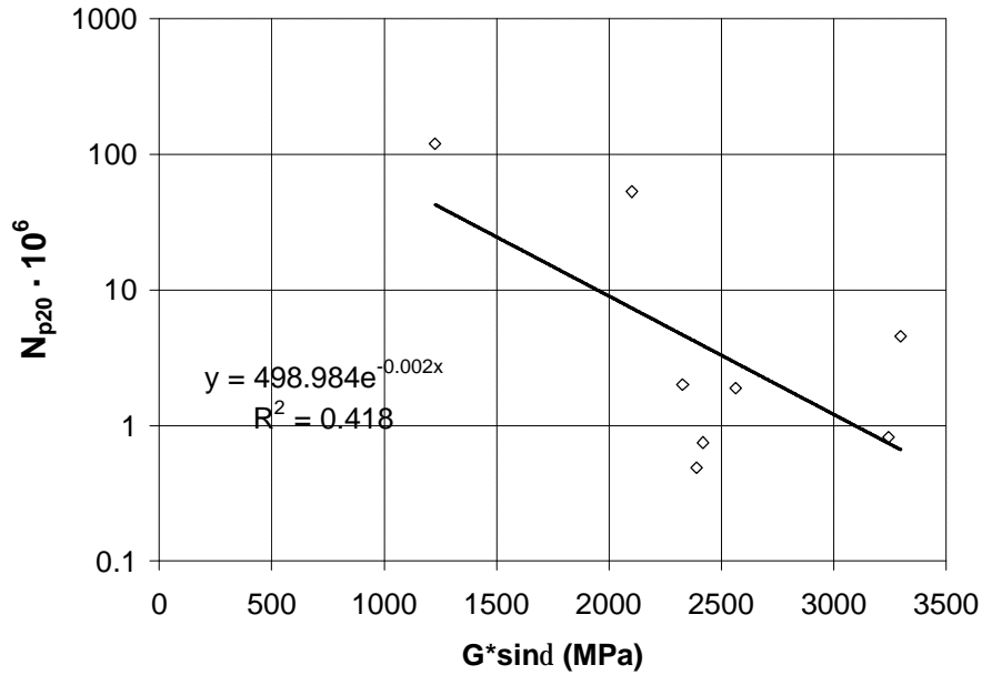
FIGURE 2.4 G \cdot \sin \delta v/s N_{p20}
