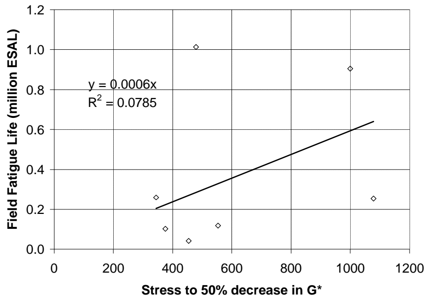
FIGURE 2.3 Stress Level to 50% decrease in G* v/s Field First Signs of Fatigue Damage
