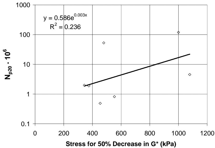
FIGURE 2.2 Stress Level to 50% decrease in G* v/s N P20
